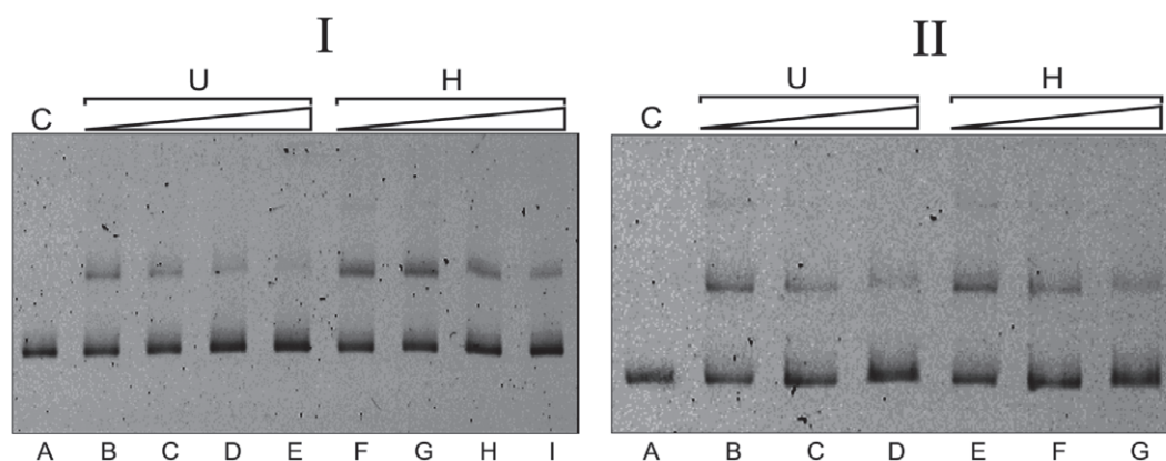
FIGURE 4. EMSA. Competition experiment demonstrating that stress-gene promoter-TBP interaction is stronger with cytosolic TBP from heat-shocked cells than for their unstressed counterparts. Panel I. Competition experiment using unlabeled vs. fluorescein-labeled J probe (DNA with the M. mazei S-6 hsp40(dnaJ) promoter). Lane A: free probe; Lanes B-E: probe incubated with extract from unstressed cells (U); Lanes F-I: probe incubated with extract from heat-shocked cells (H). C: competitor added, none ( lanes B and F ), 2 μl ( lanes C and G ), 4 μl ( lanes D and H ), and 8 μl ( lanes E and I ). Panel II. Competition experiments using unlabeled 29-mer bearing the hsp70(dnaK) promoter vs. fluorescein-labeled J probe; the EMSA was carried out with the latter, as in Panel I. Lane A: free probe; Lanes B-D: probe incubated with extract from unstressed cells (U); Lanes E-G: probe incubated with extract from heat-shocked cells (H). C: competitor added, none ( lanes B and E ), 2 μl ( lanes C and F ), and 4 μl ( lanes D and G ). (Reproduced from De Biase et al., 2002, with permission.)
